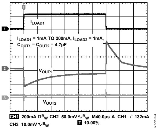
Figure 24. Load Transient Response, I_{LOAD1} = 1mA to 200mA , I_{LOAD2} = 1mA , C_{OUT1} = C_{OUT2} = 4.7µF CH1 = I_{LOAD1} , CH2 = V_{OUT1} , CH3 = V_{OUT2}
