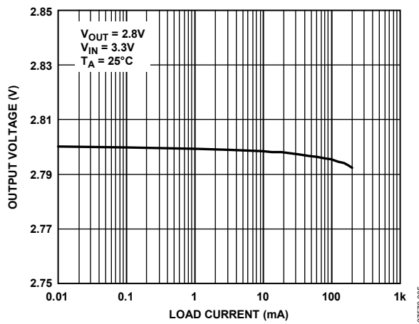
Figure 5. Output Voltage vs. Load Current
