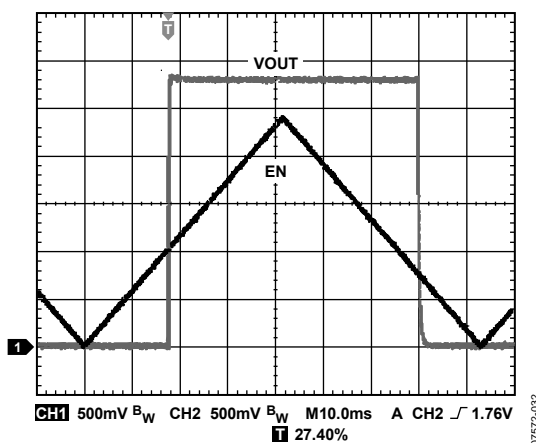
Figure 32. Typical EN Pin Operation
